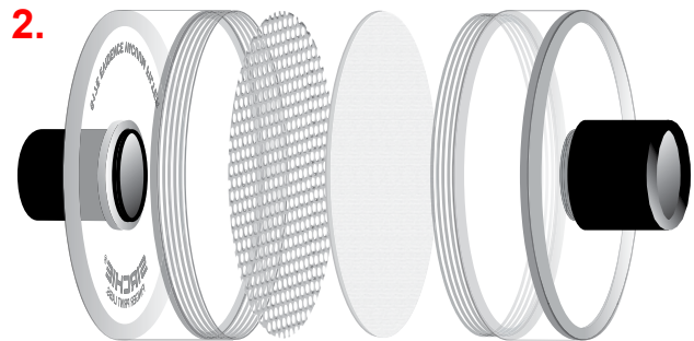
PEM01 Microfilter Installation
