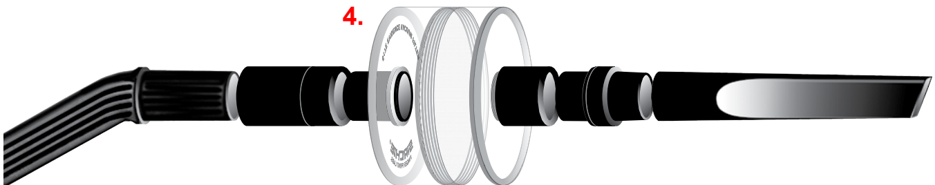
617E Assembly using Adapters for Tool and Hose Attachment
